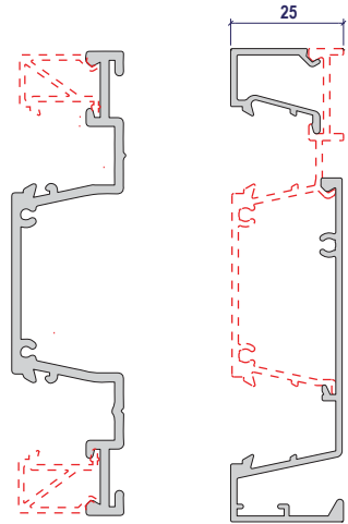
AE041 Frontline double glazing track
